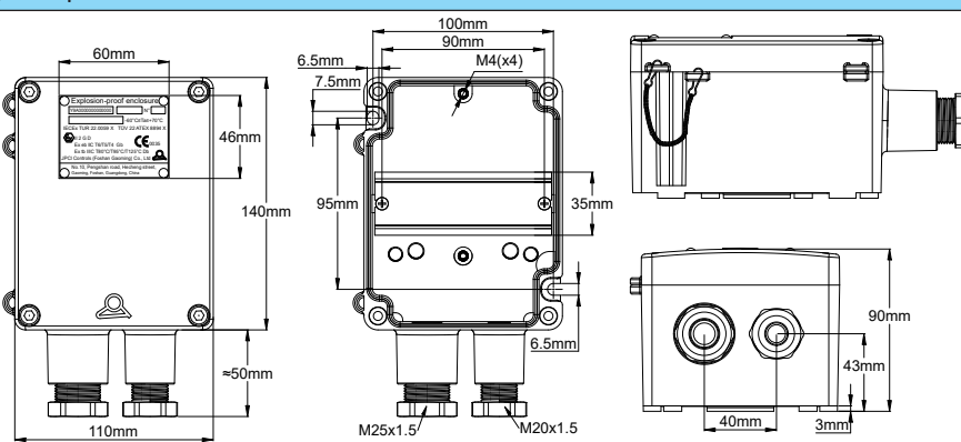
Example with only DIN rail
